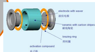
多間隙高能GDT Multi-gap high voltage GDT
